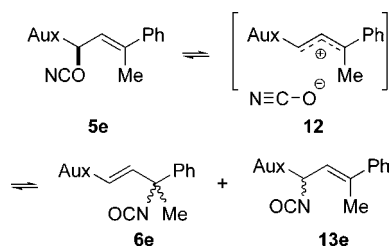
Figure 3. Possible cationic intermediates.
