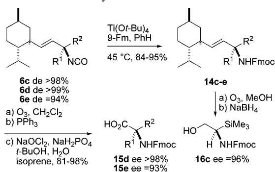
Scheme 2. Synthesis of α-Amino Acids 15
