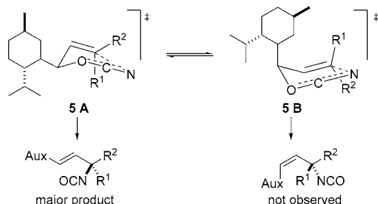
Figure 2. Possible transition states for the rearrangement.
