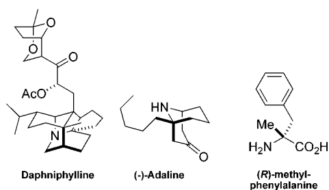
Figure 1. Natural products containing a quaternary chiral carbon bearing nitrogen.
